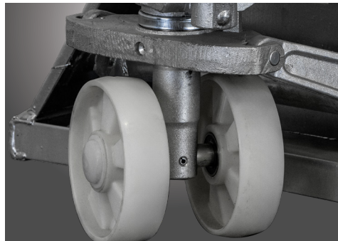
White nylon steer wheels and load rollers complete with shielded ball bearings.
